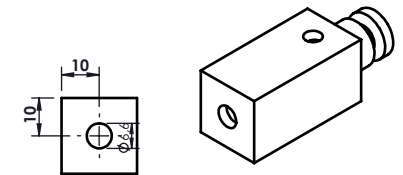
Bracket Assembly
