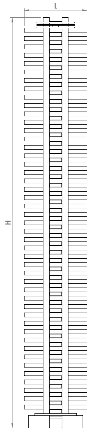
Front View
